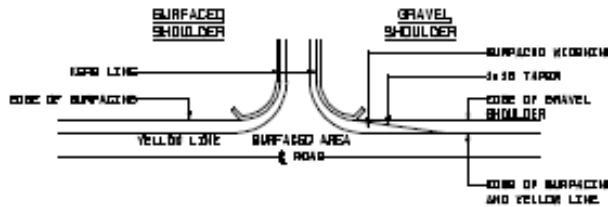
KERBED INTERSECTION
