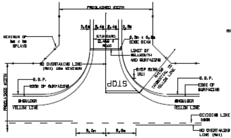
THROUGH ROAD INTERSECTION WITH CLASS 4 ROAD OR MAJOR PRIVATE ACCESS
