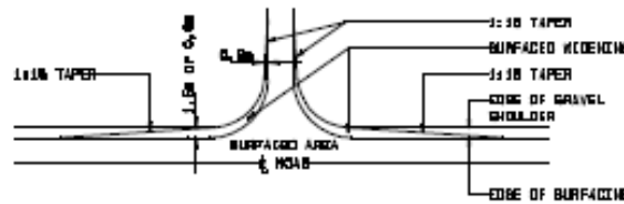
INTERSECTION OF SURFACED ROADS
