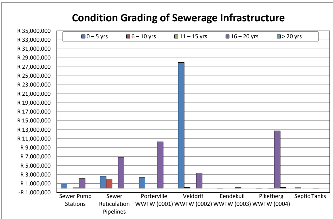
Figure C.6.8: Condition grading of the sewerage infrastructure
