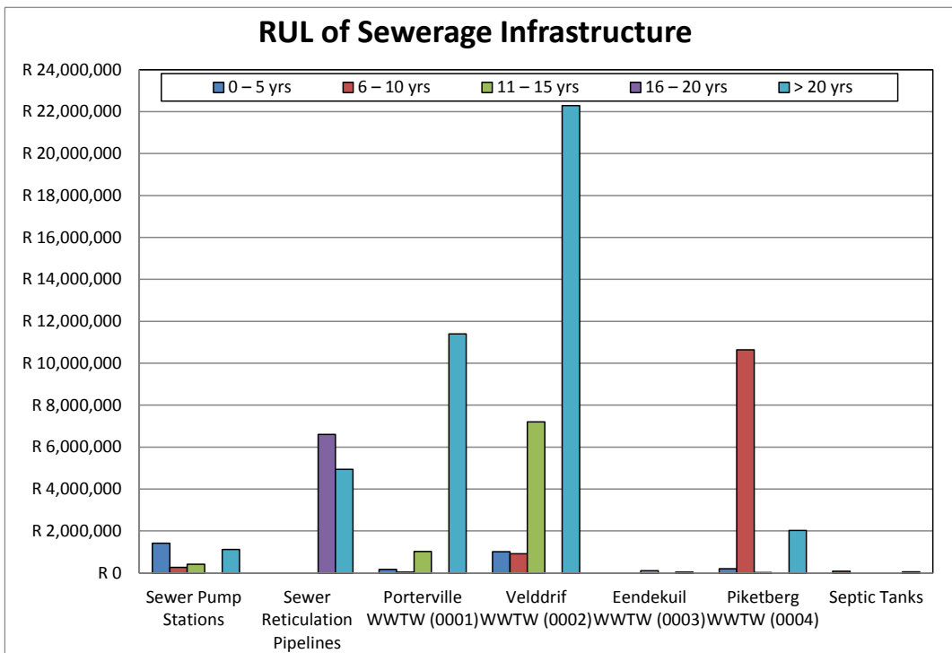
Figure C.6.6: Remaining Useful Life of the sewerage infrastructure
