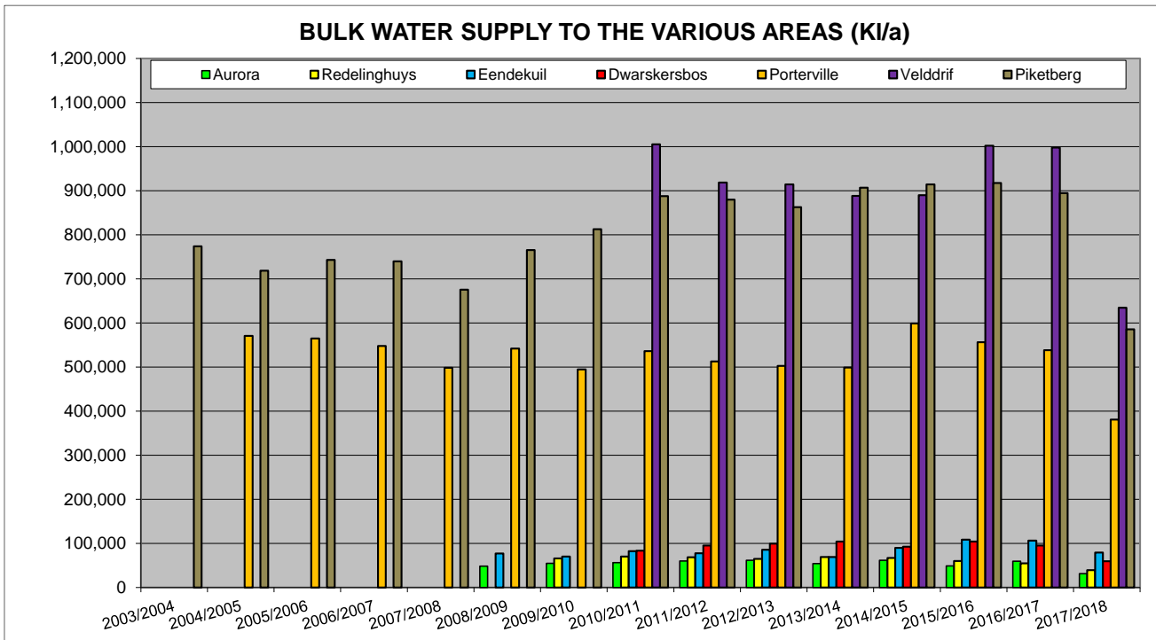
Figure C.1.1: Bulk water supply for the various distribution systems
